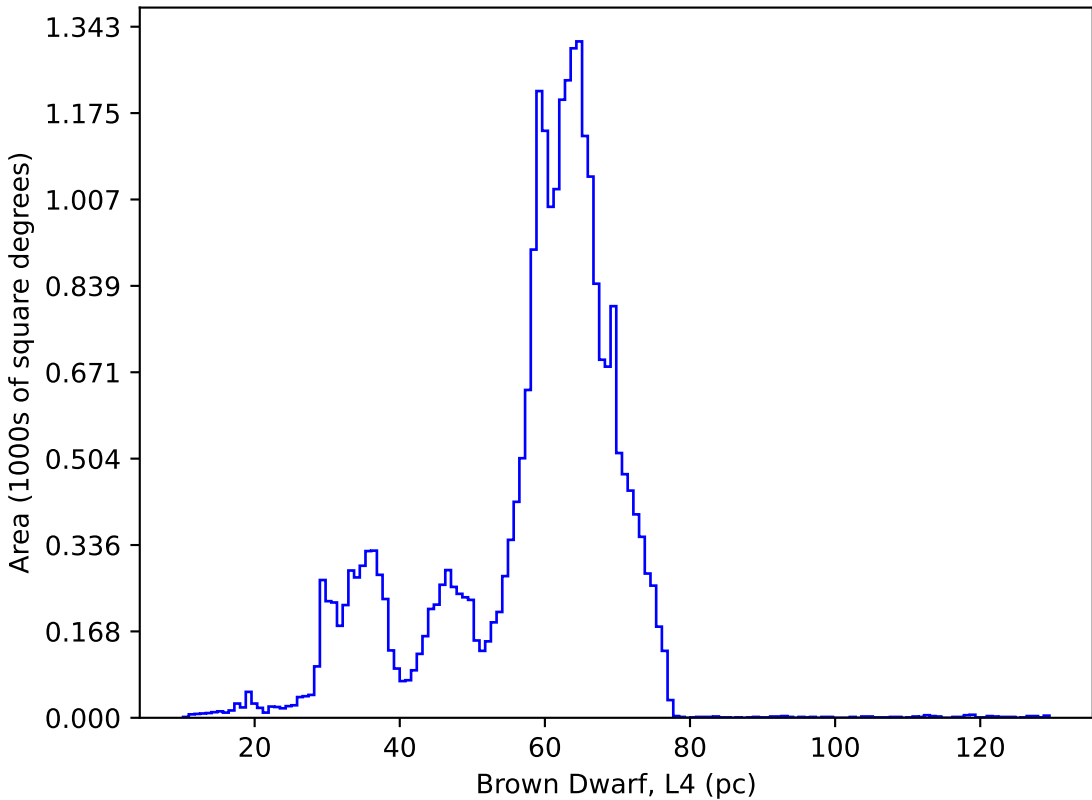
internal_u_expt60_nscale1.1v3.4_10yrs : Brown Dwarf, L4
