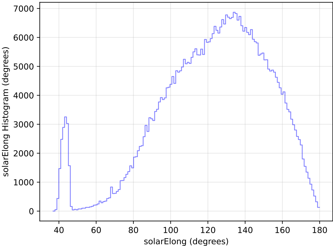
internal_u_expt60_nscale1.1v3.4_10yrs WFD r band: solarElong Histogram
