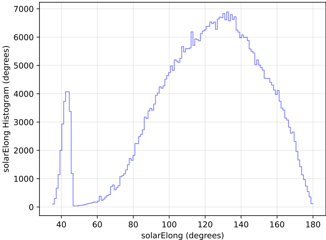
internal_u_expt60_nscale1.1v3.4_10yrs WFD i band: solarElong Histogram
