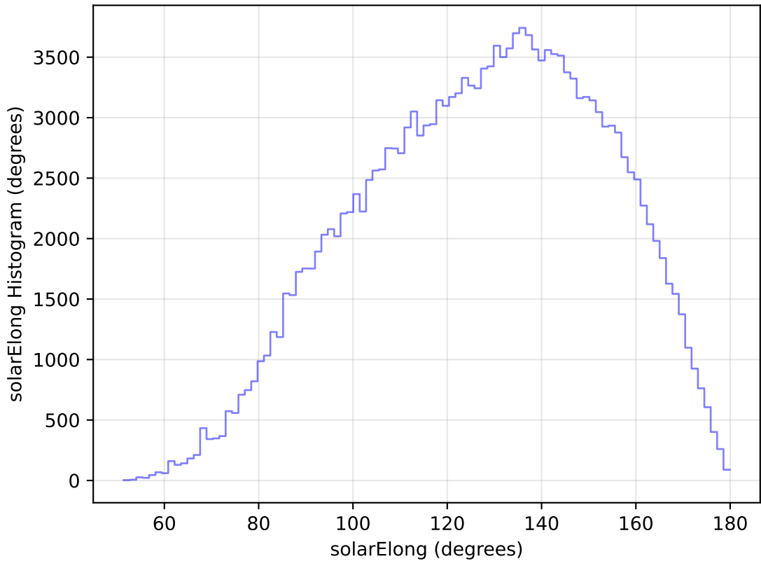
internal_u_expt60_nscale1.1v3.4_10yrs WFD g band: solarElong Histogram
