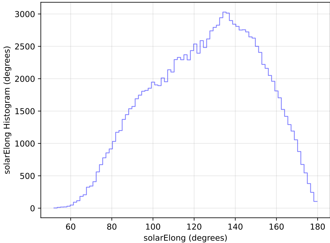
internal_u_expt60_nscale1.1v3.4_10yrs All sky u band: solarElong Histogram
