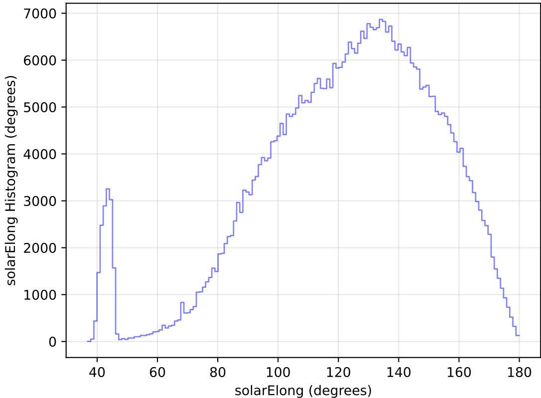
internal_u_expt60_nscale1.1v3.4_10yrs All sky r band: solarElong Histogram
