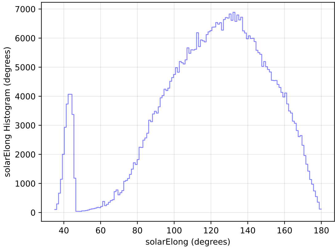
internal_u_expt60_nscale1.1v3.4_10yrs All sky i band: solarElong Histogram
