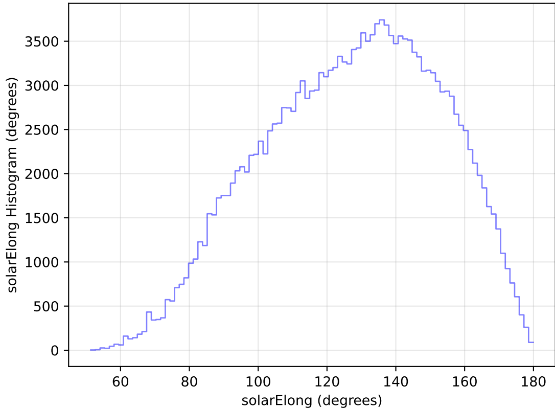
internal_u_expt60_nscale1.1v3.4_10yrs All sky g band: solarElong Histogram
