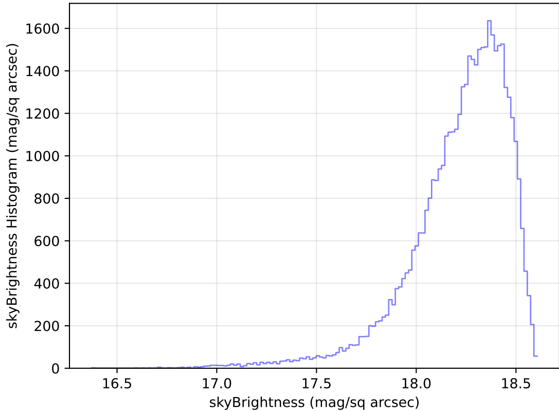
internal_u_expt60_nscale1.1v3.4_10yrs Yr 1 y band: skyBrightness Histogram
