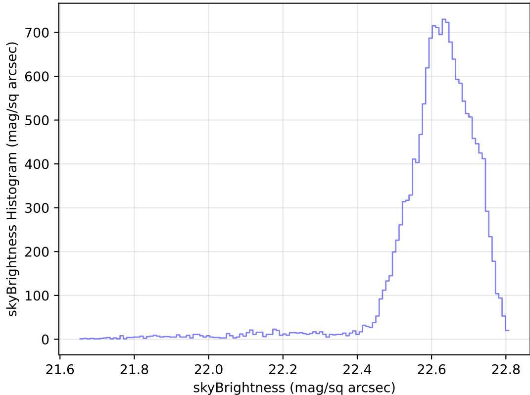
internal_u_expt60_nscale1.1v3.4_10yrs Yr 1 u band: skyBrightness Histogram
