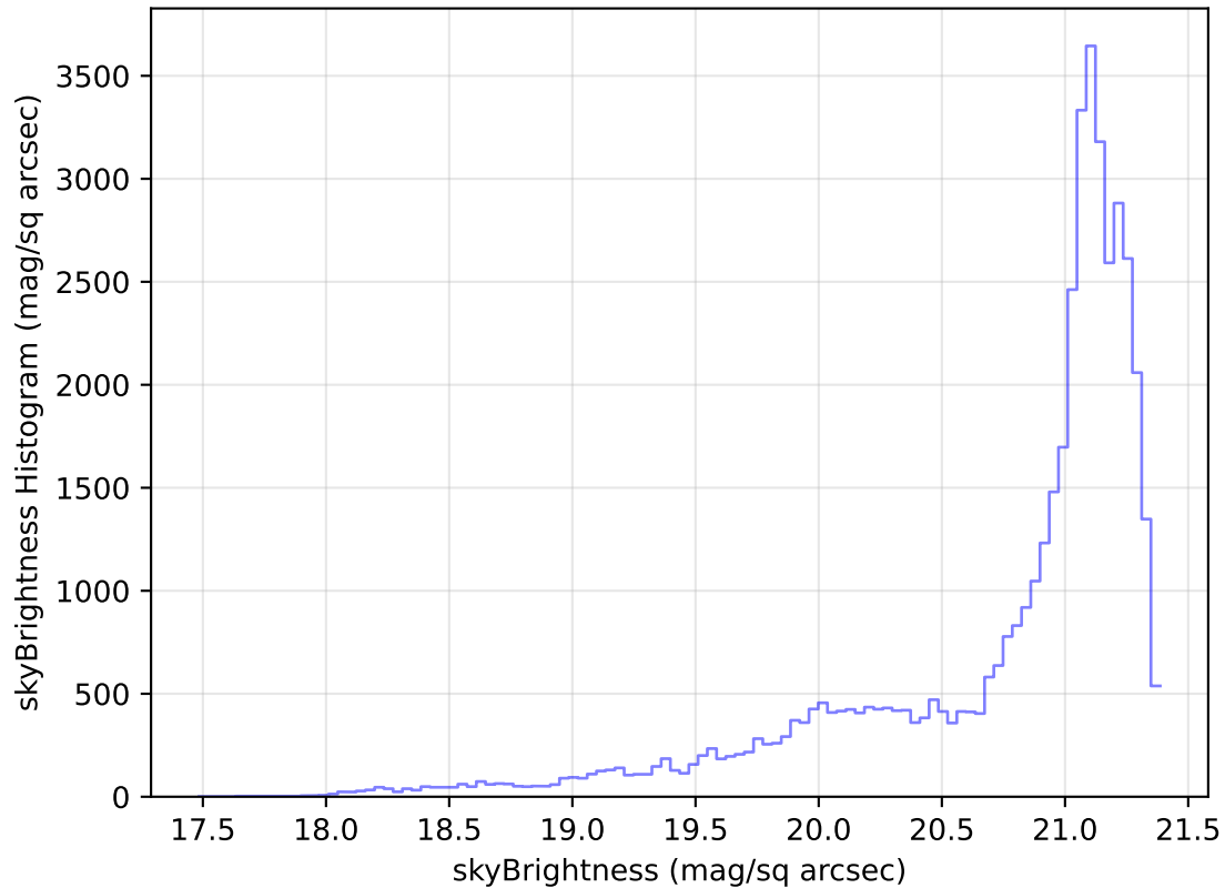
internal_u_expt60_nscale1.1v3.4_10yrs Yr 1 r band: skyBrightness Histogram
