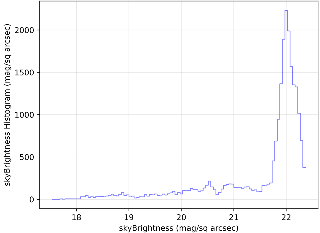
internal_u_expt60_nscale1.1v3.4_10yrs Yr 1 g band: skyBrightness Histogram
