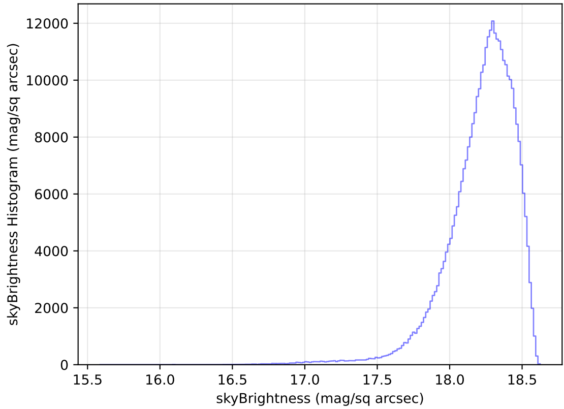
internal_u_expt60_nscale1.1v3.4_10yrs WFD y band: skyBrightness Histogram
