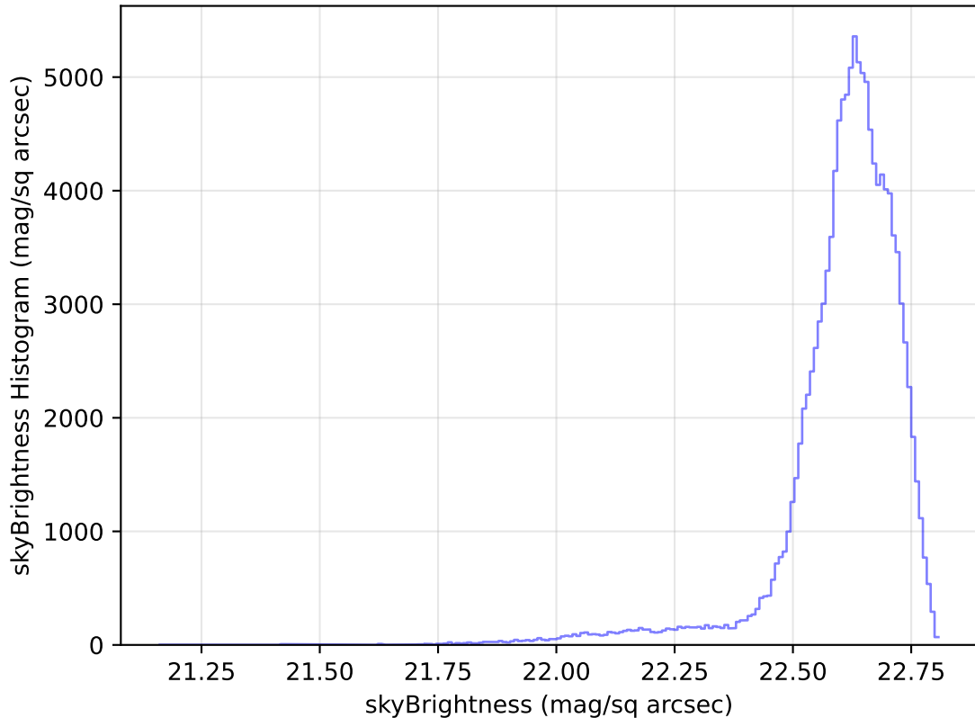
internal_u_expt60_nscale1.1v3.4_10yrs WFD u band: skyBrightness Histogram
