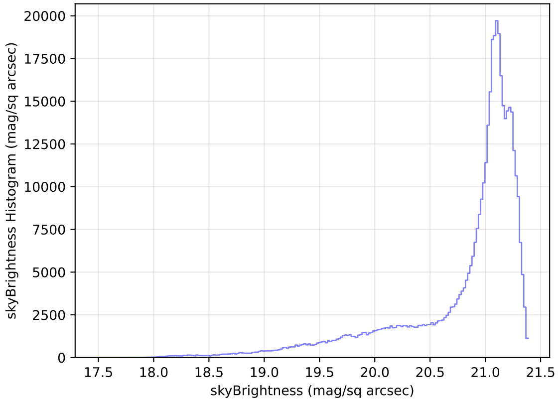
internal_u_expt60_nscale1.1v3.4_10yrs WFD r band: skyBrightness Histogram
