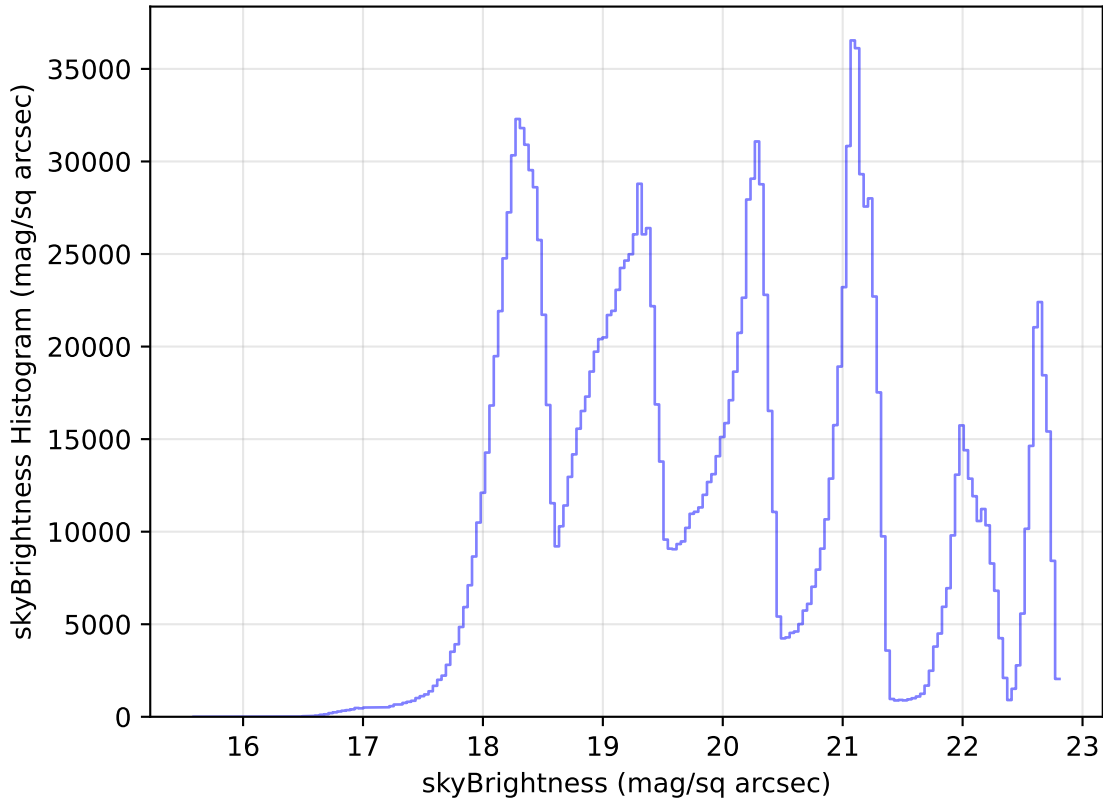
internal_u_expt60_nscale1.1v3.4_10yrs WFD all bands: skyBrightness Histogram
