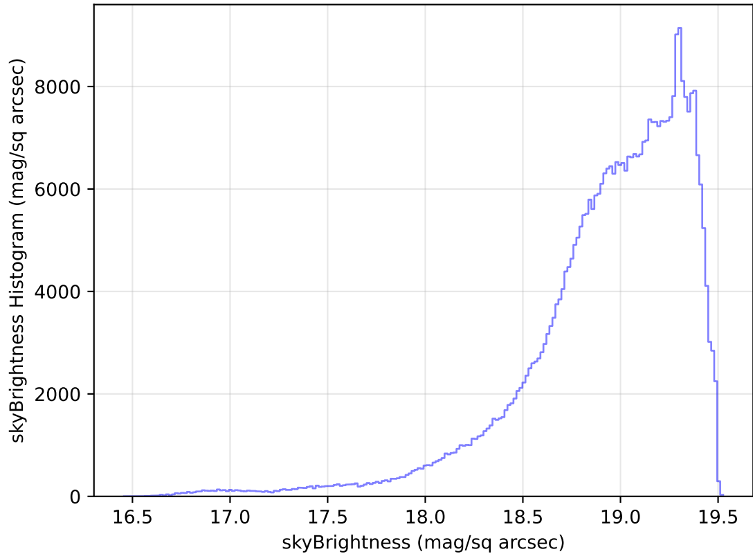
internal_u_expt60_nscale1.1v3.4_10yrs All sky z band: skyBrightness Histogram
