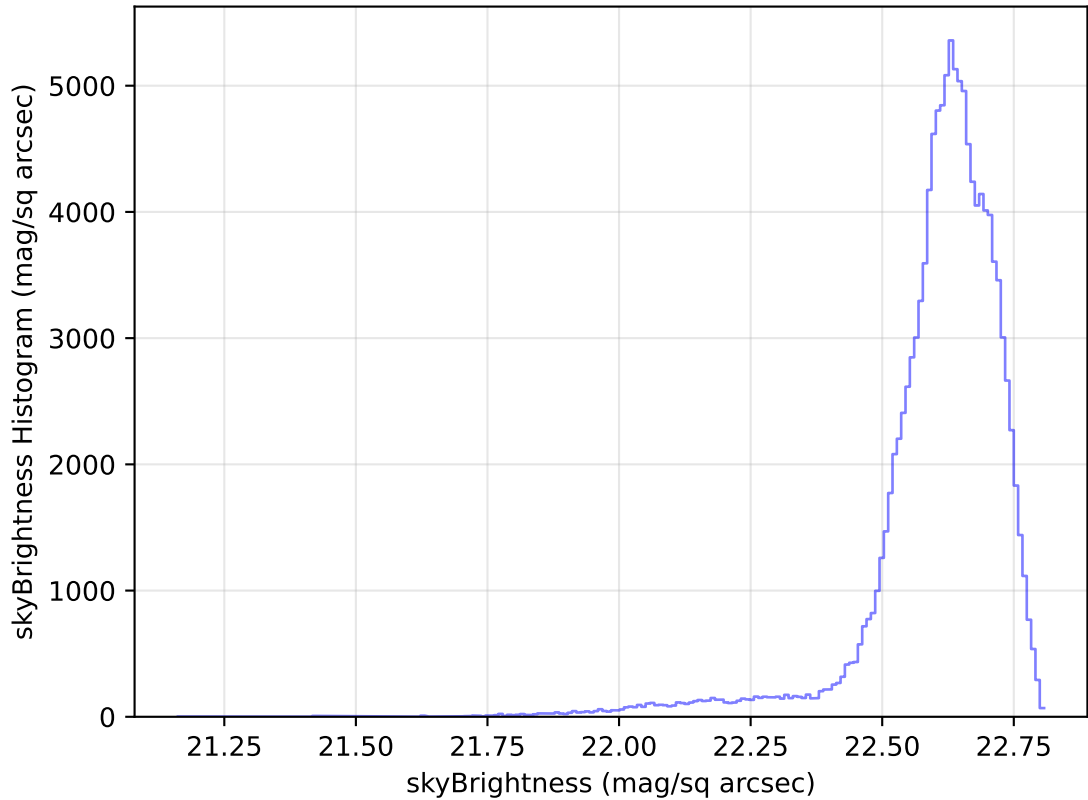
internal_u_expt60_nscale1.1v3.4_10yrs All sky u band: skyBrightness Histogram
