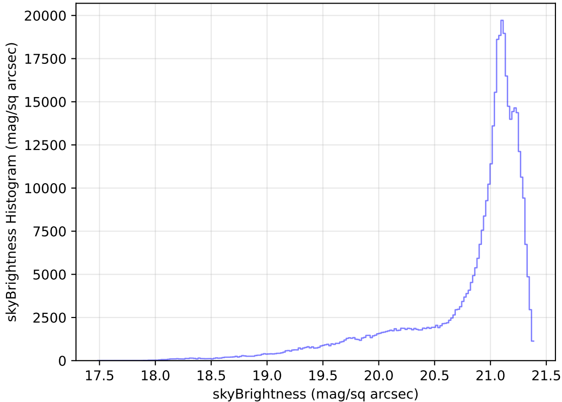
internal_u_expt60_nscale1.1v3.4_10yrs All sky r band: skyBrightness Histogram
