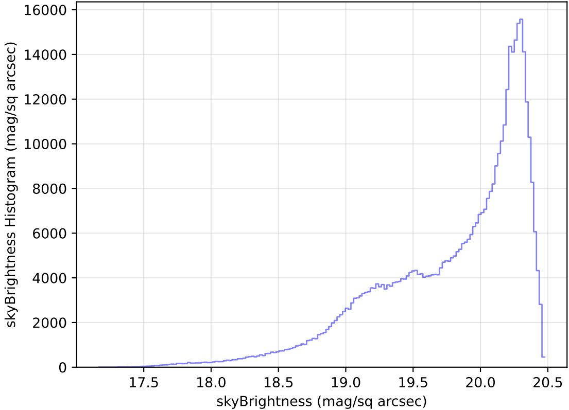
internal_u_expt60_nscale1.1v3.4_10yrs All sky i band: skyBrightness Histogram
