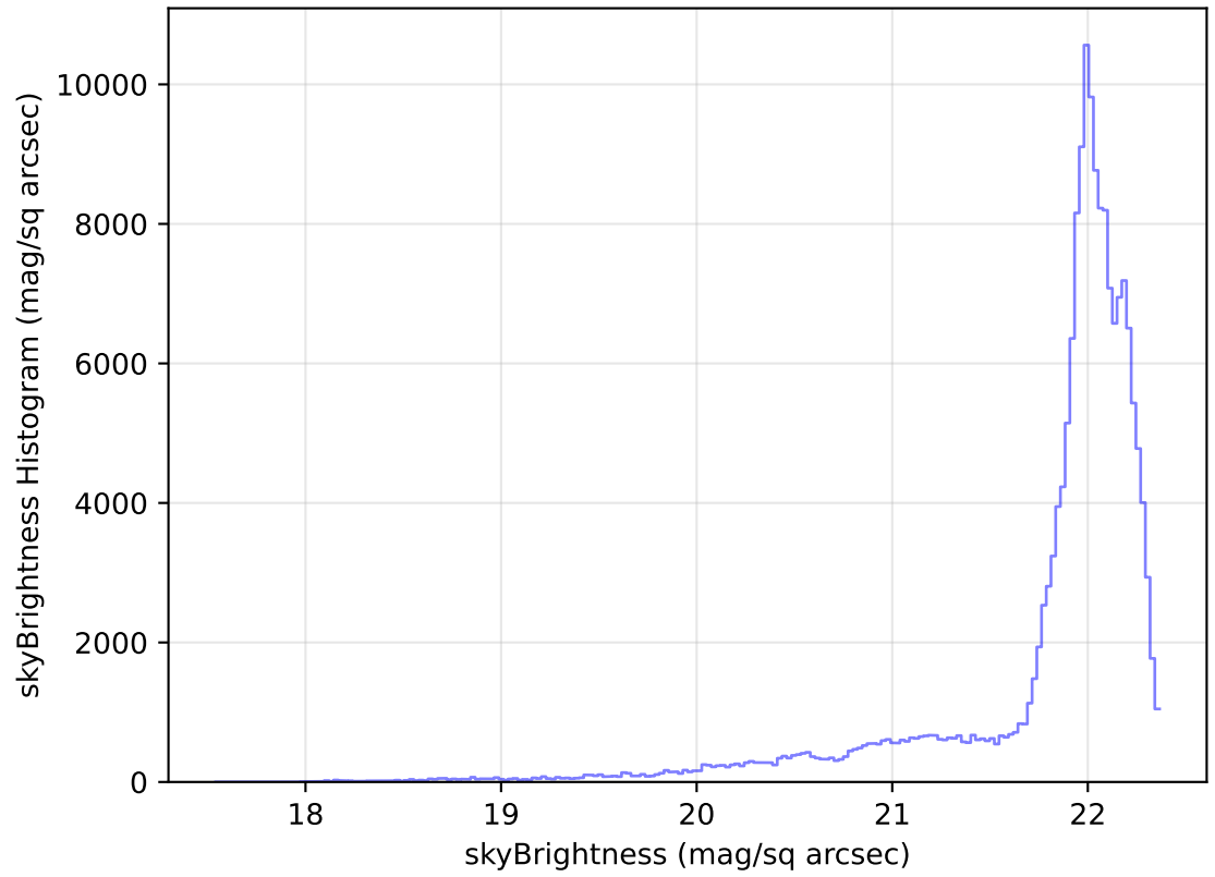
internal_u_expt60_nscale1.1v3.4_10yrs All sky g band: skyBrightness Histogram
