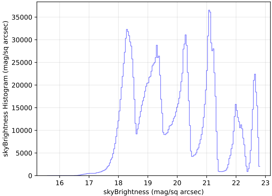
internal_u_expt60_nscale1.1v3.4_10yrs All sky all bands: skyBrightness Histogram
