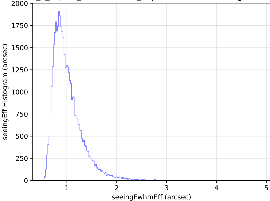
internal_u_expt60_nscale1.1v3.4_10yrs Yr 1 z band: seeingEff Histogram
