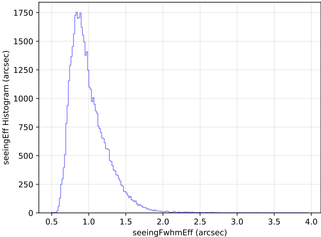
internal_u_expt60_nscale1.1v3.4_10yrs Yr 1 y band: seeingEff Histogram
