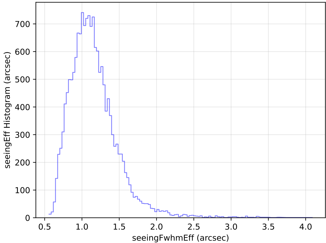
internal_u_expt60_nscale1.1v3.4_10yrs Yr 1 u band: seeingEff Histogram
