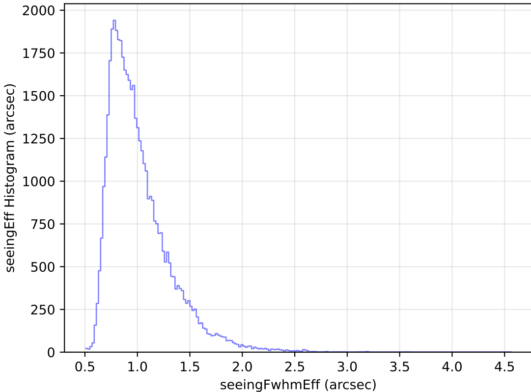
internal_u_expt60_nscale1.1v3.4_10yrs Yr 1 r band: seeingEff Histogram
