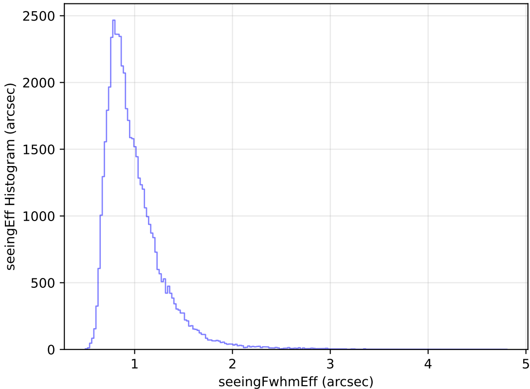
internal_u_expt60_nscale1.1v3.4_10yrs Yr 1 i band: seeingEff Histogram
