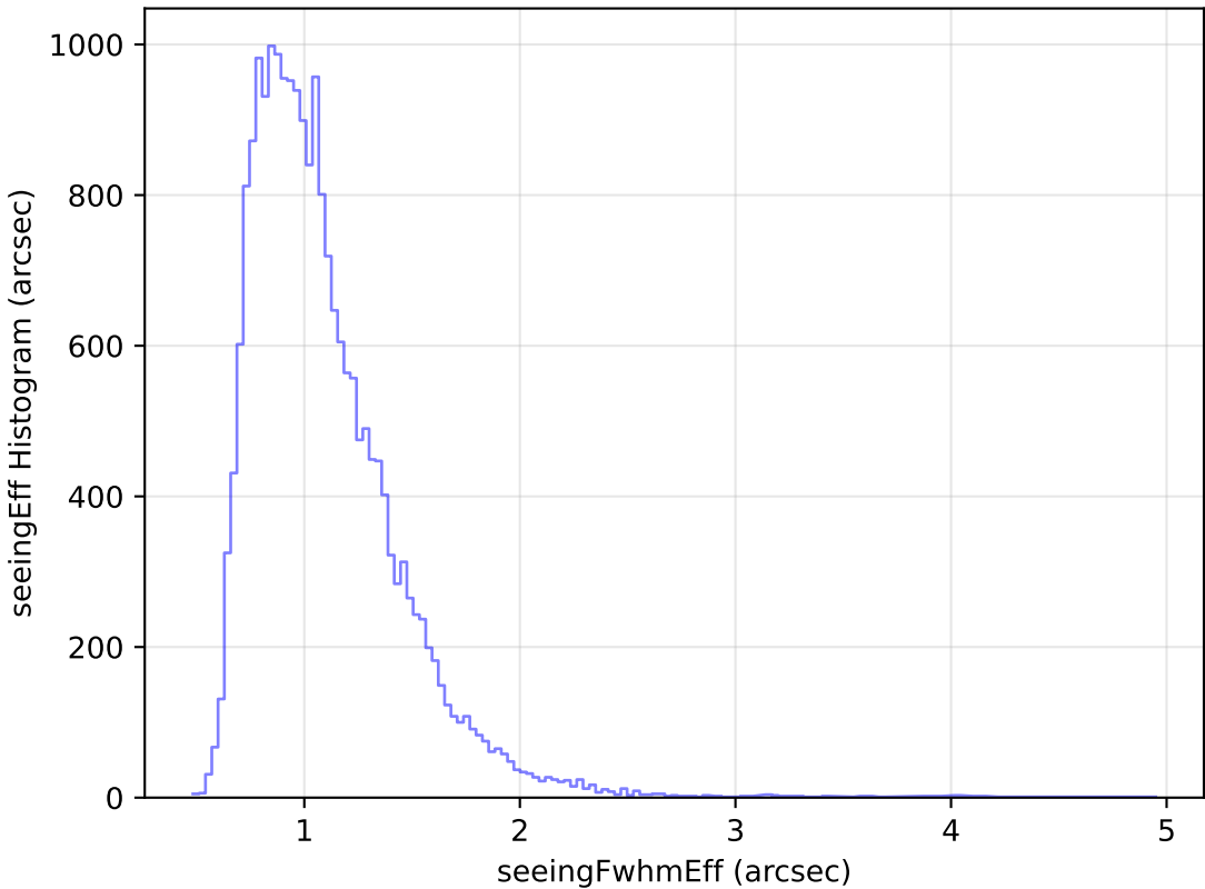
internal_u_expt60_nscale1.1v3.4_10yrs Yr 1 g band: seeingEff Histogram
