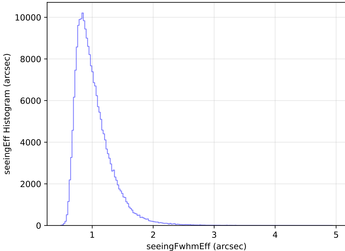
internal_u_expt60_nscale1.1v3.4_10yrs Yr 1 all bands: seeingEff Histogram
