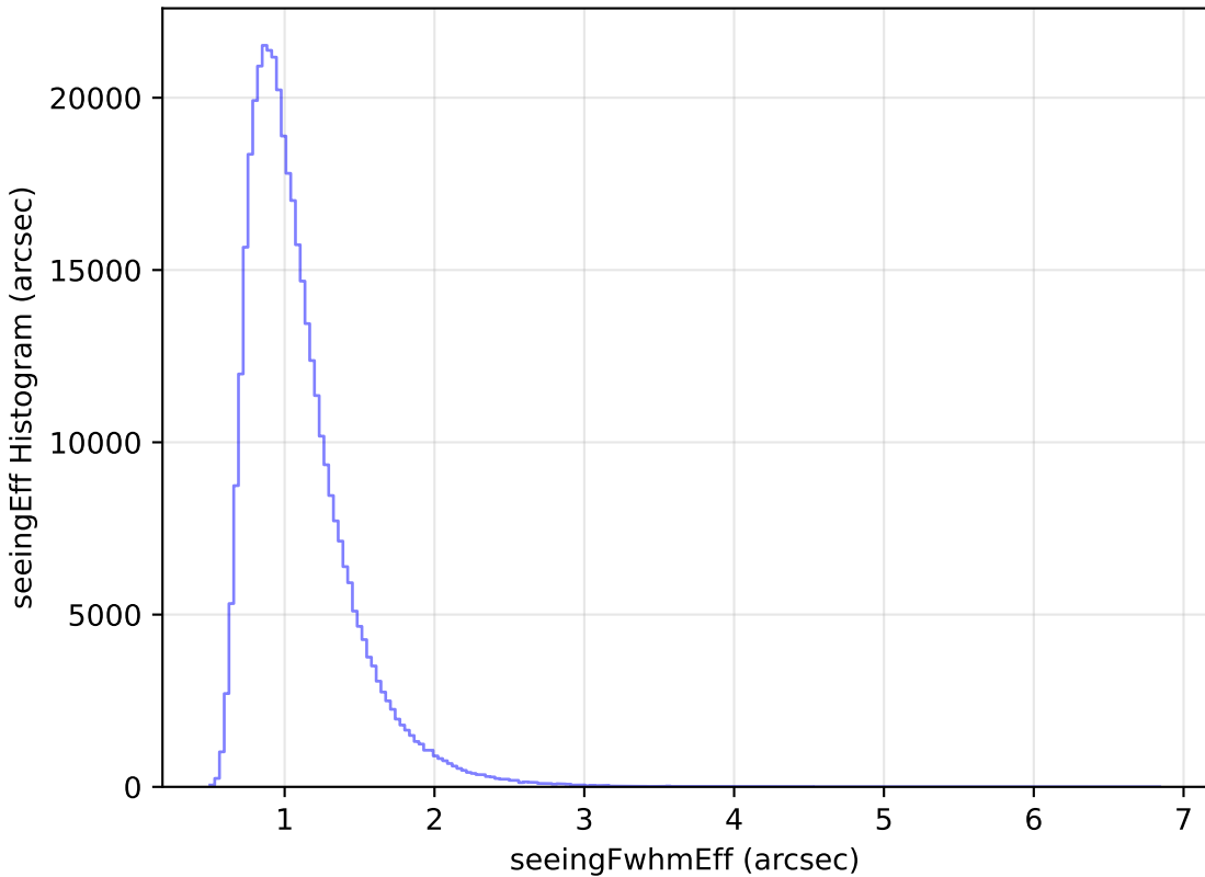
internal_u_expt60_nscale1.1v3.4_10yrs WFD z band: seeingEff Histogram
