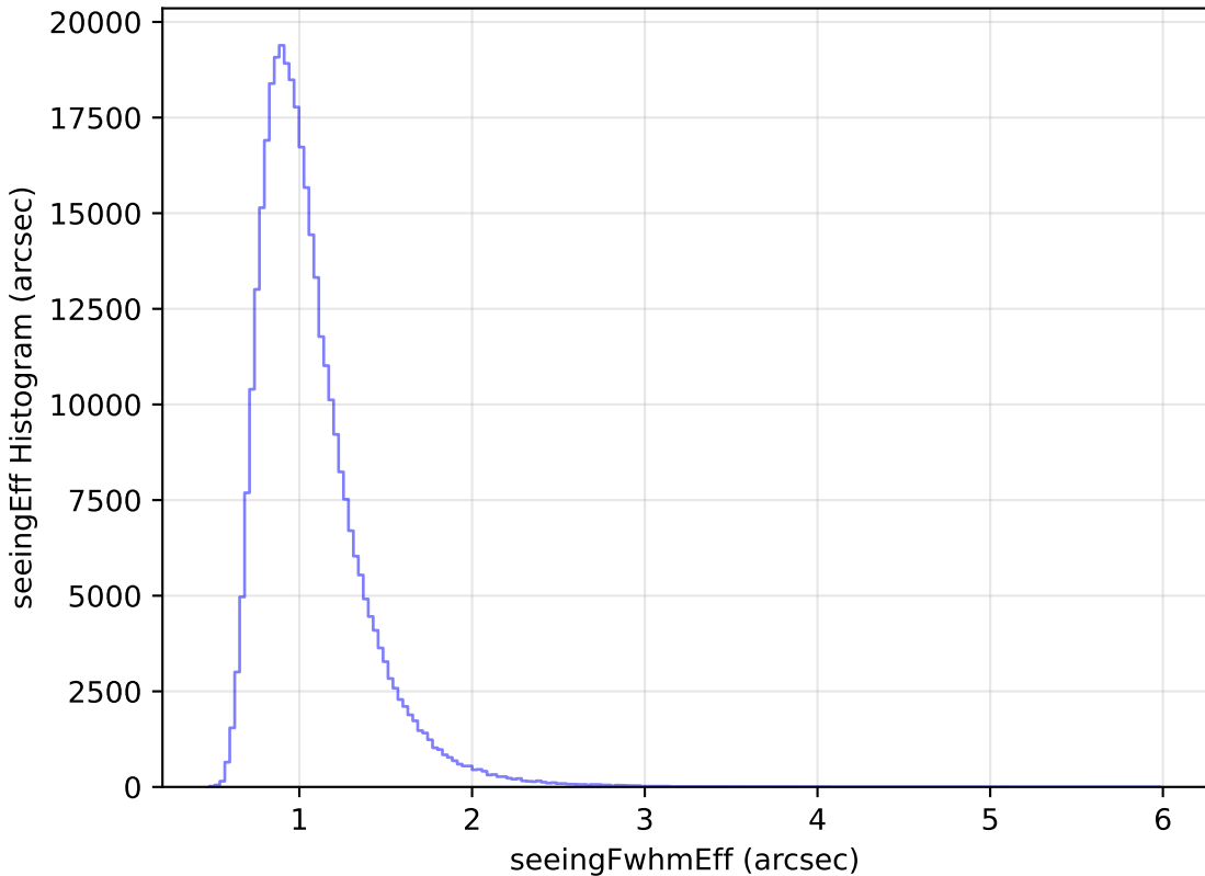
internal_u_expt60_nscale1.1v3.4_10yrs WFD y band: seeingEff Histogram
