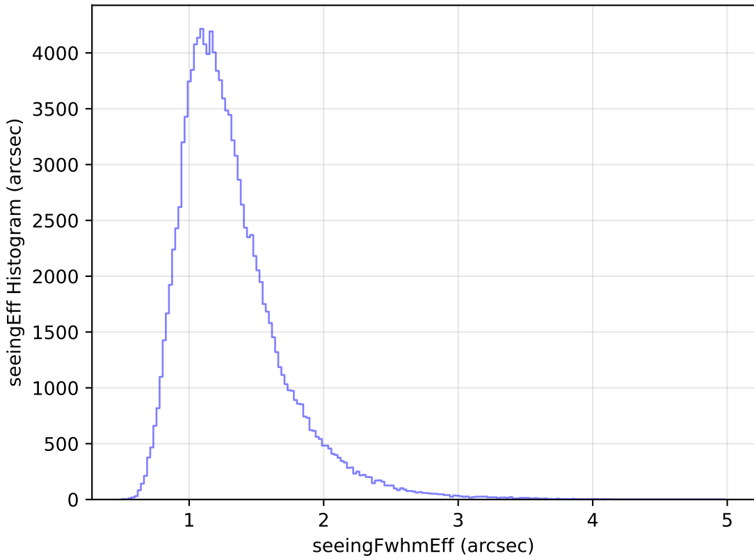
internal_u_expt60_nscale1.1v3.4_10yrs WFD u band: seeingEff Histogram
