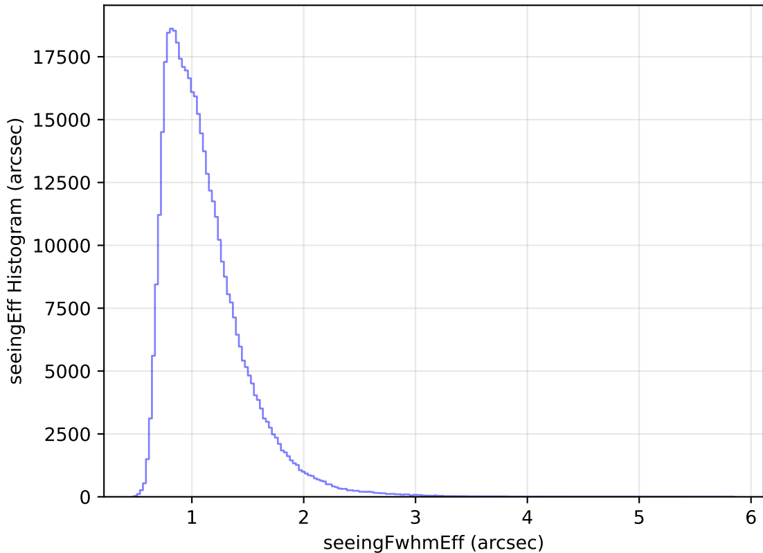
internal_u_expt60_nscale1.1v3.4_10yrs WFD r band: seeingEff Histogram
