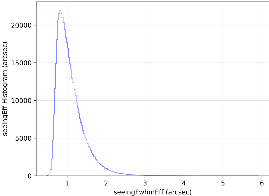
internal_u_expt60_nscale1.1v3.4_10yrs WFD i band: seeingEff Histogram
