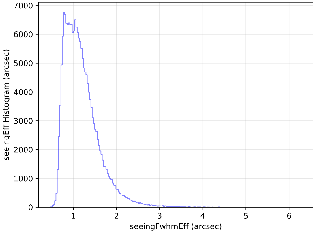
internal_u_expt60_nscale1.1v3.4_10yrs WFD g band: seeingEff Histogram
