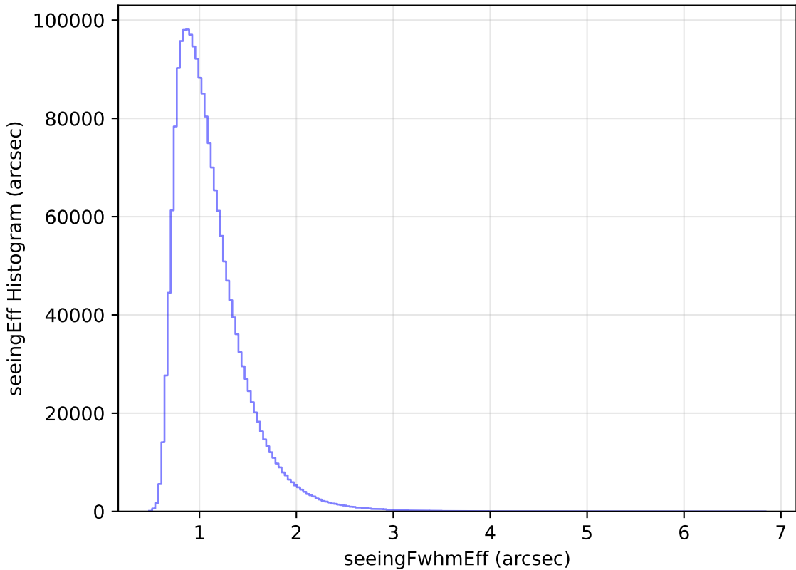
internal_u_expt60_nscale1.1v3.4_10yrs WFD all bands: seeingEff Histogram
