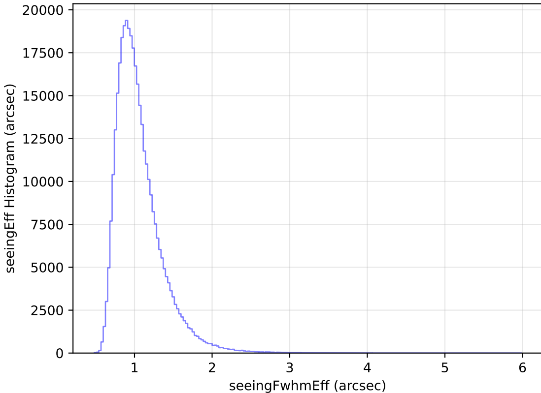
internal_u_expt60_nscale1.1v3.4_10yrs All sky y band: seeingEff Histogram
