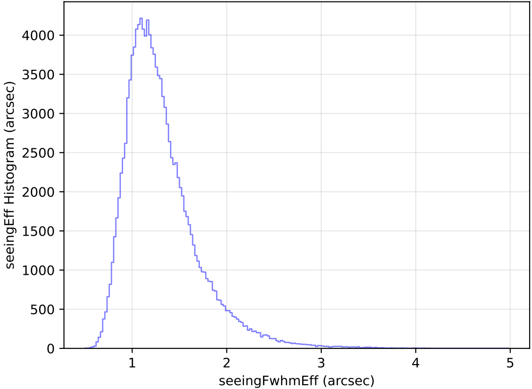
internal_u_expt60_nscale1.1v3.4_10yrs All sky u band: seeingEff Histogram
