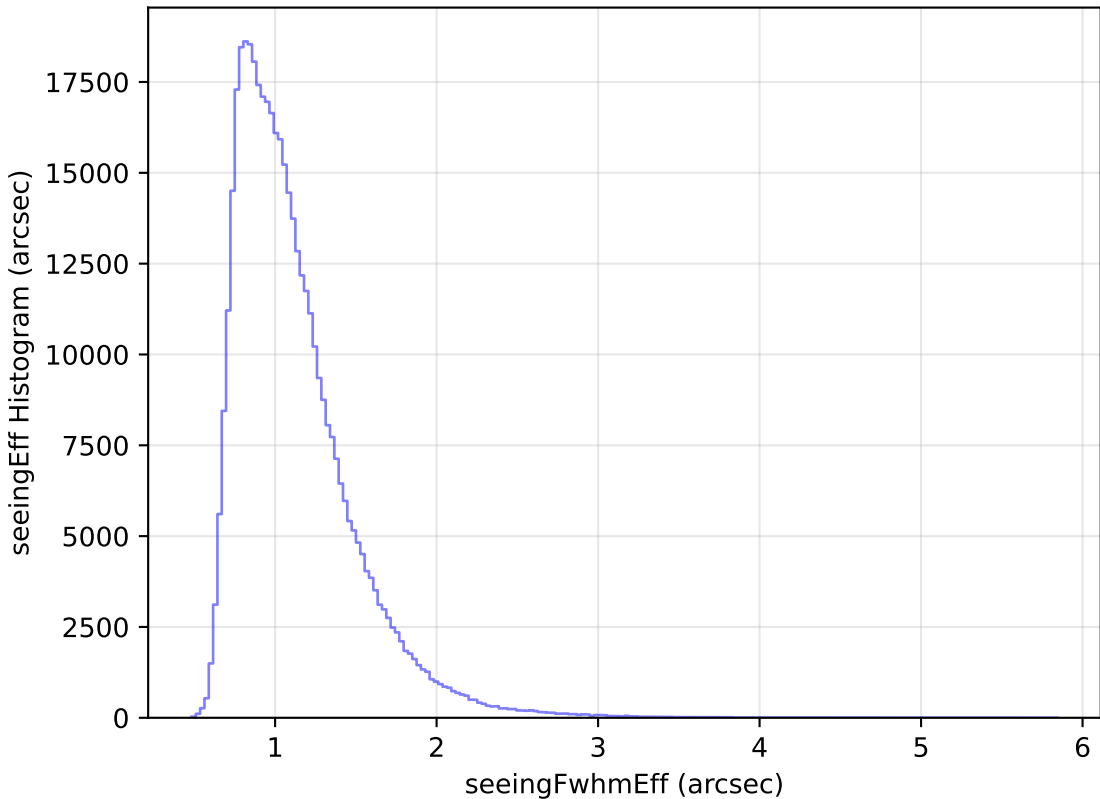
internal_u_expt60_nscale1.1v3.4_10yrs All sky r band: seeingEff Histogram
