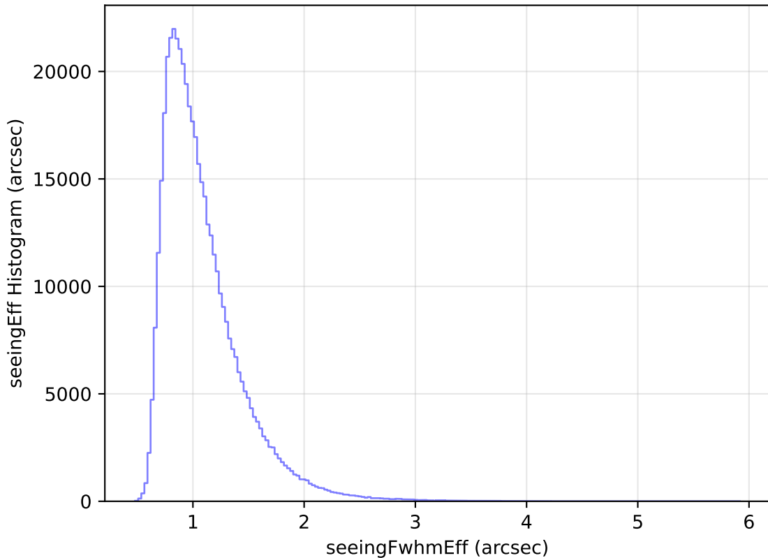
internal_u_expt60_nscale1.1v3.4_10yrs All sky i band: seeingEff Histogram
