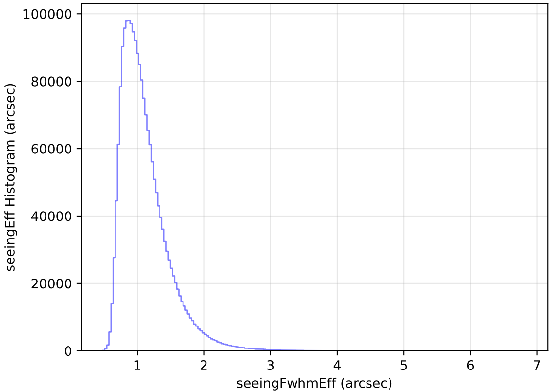
internal_u_expt60_nscale1.1v3.4_10yrs All sky all bands: seeingEff Histogram
