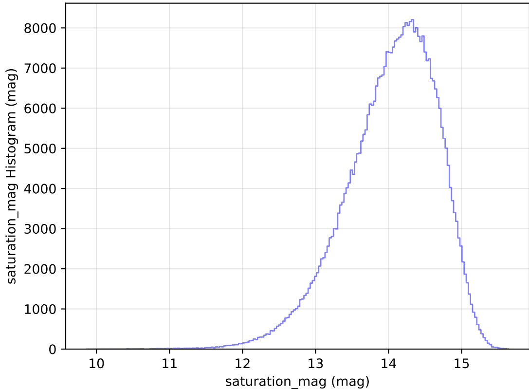
internal_u_expt60_nscale1.1v3.4_10yrs WFD z band: saturation_mag Histogram
