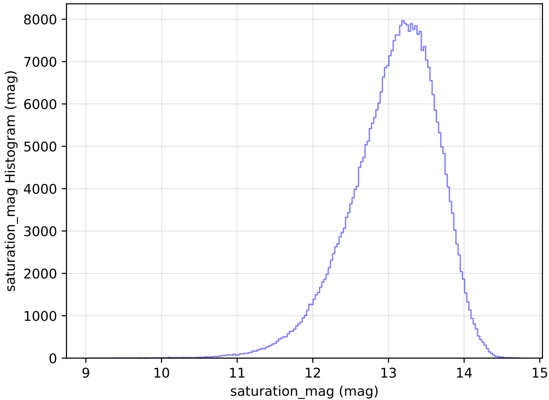
internal_u_expt60_nscale1.1v3.4_10yrs WFD y band: saturation_mag Histogram
