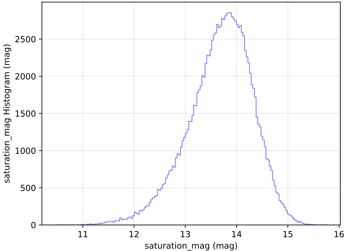
internal_u_expt60_nscale1.1v3.4_10yrs WFD u band: saturation_mag Histogram
