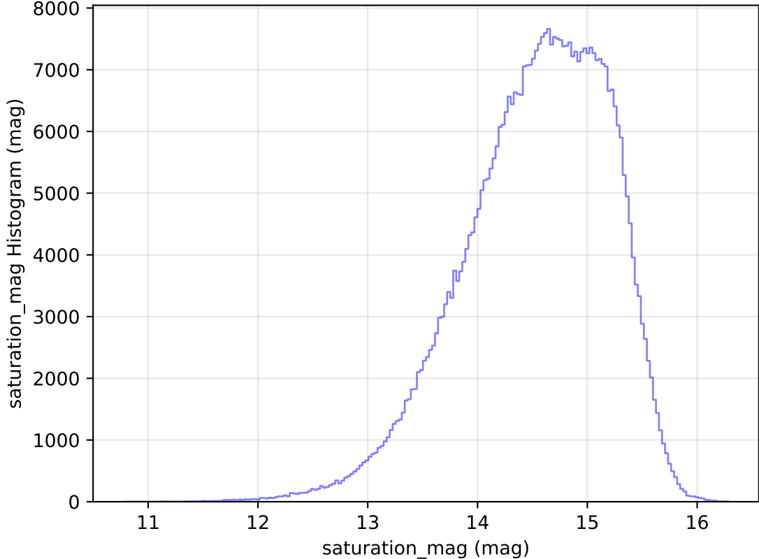
internal_u_expt60_nscale1.1v3.4_10yrs WFD r band: saturation_mag Histogram
