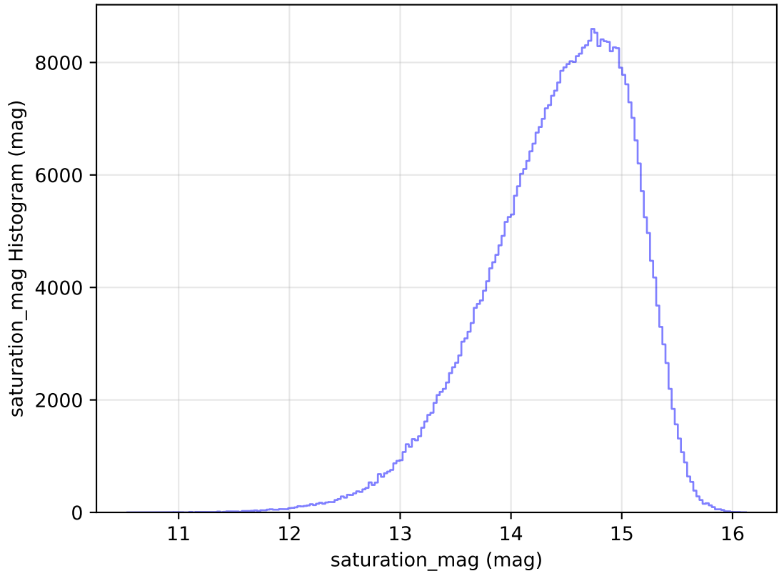
internal_u_expt60_nscale1.1v3.4_10yrs WFD i band: saturation_mag Histogram
