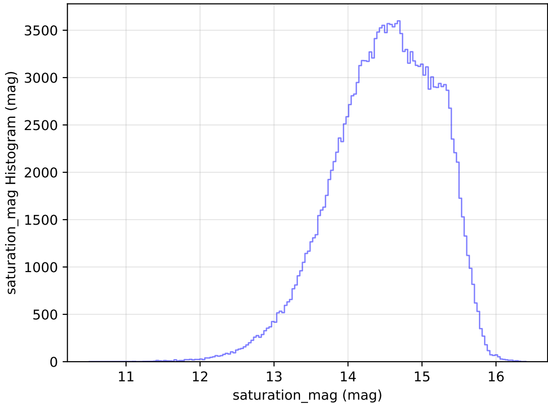
internal_u_expt60_nscale1.1v3.4_10yrs WFD g band: saturation_mag Histogram
