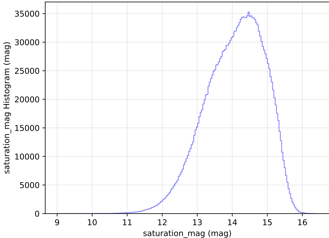
internal_u_expt60_nscale1.1v3.4_10yrs WFD all bands: saturation_mag Histogram
