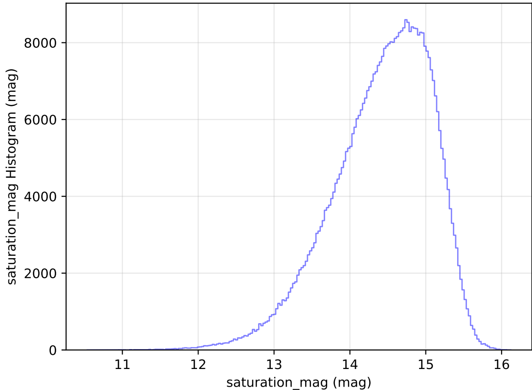
internal_u_expt60_nscale1.1v3.4_10yrs All sky i band: saturation_mag Histogram
