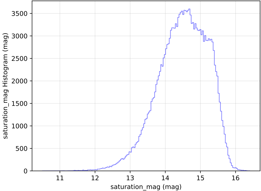
internal_u_expt60_nscale1.1v3.4_10yrs All sky g band: saturation_mag Histogram
